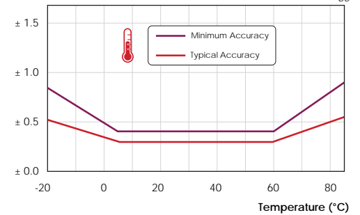
Accuracy (%RH)
