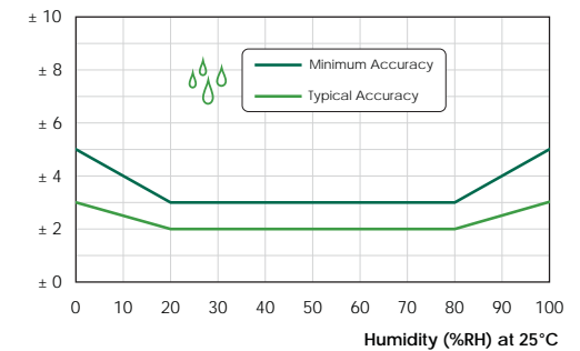
Accuracy (%RH)
