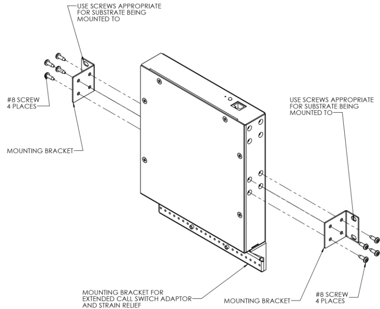
Figure 1. Wall Mounting
